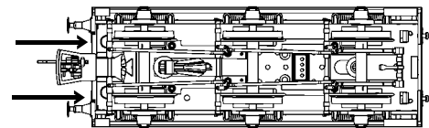
Remove tender body securing screws
